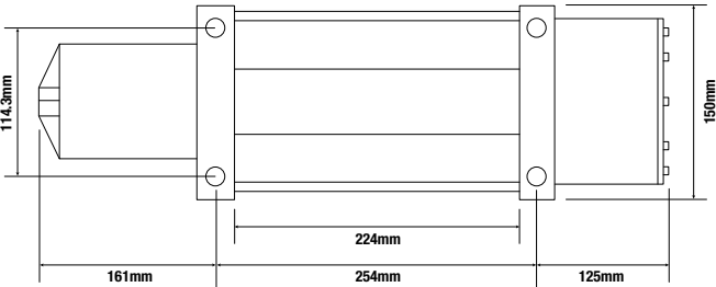
BOLTING PATTERN
